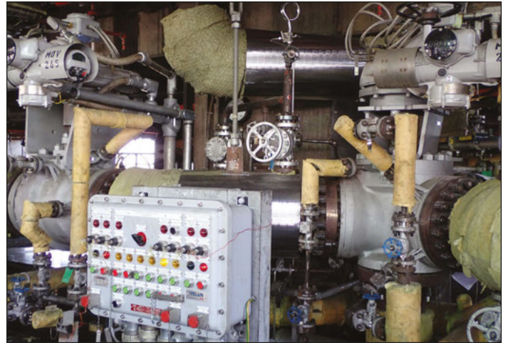
One of Velan's Severe Service Strategic Business Unit's (SBU) customer-centric offerings this year included three actuated Securaseal metal-seated ball valves, a Programmable Logic Controller (PLC), and local control panels into a single factory-tested package installed in one of the newest delayed coking units in the world.
