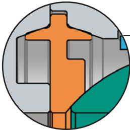
Downstream seat Up To 6" (150 mm)
